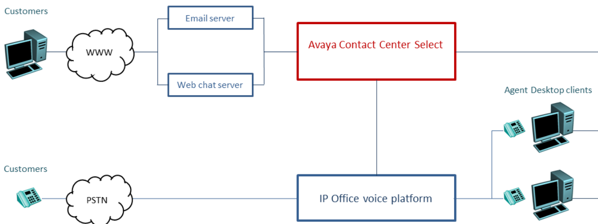
Figure 7: Typical contact center solution using voice and multimedia Avaya Contact Center Select and the Avaya IP Office voice phone system
